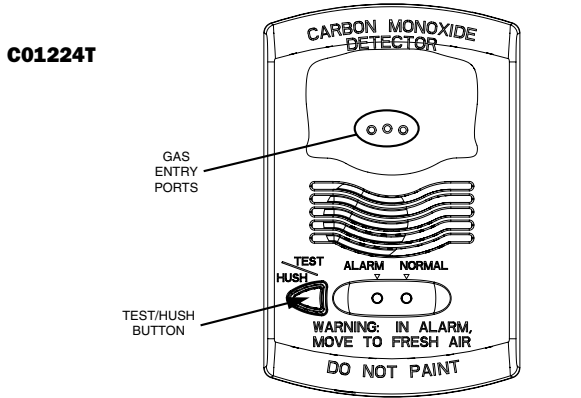
FIGURE 4. TEST BUTTON LOCATION AND OPERATION:
